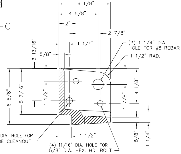
SECTION B-B
